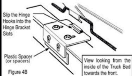
Approx. Bracket Location Shown -Remove it Prior to Marking Bed-
