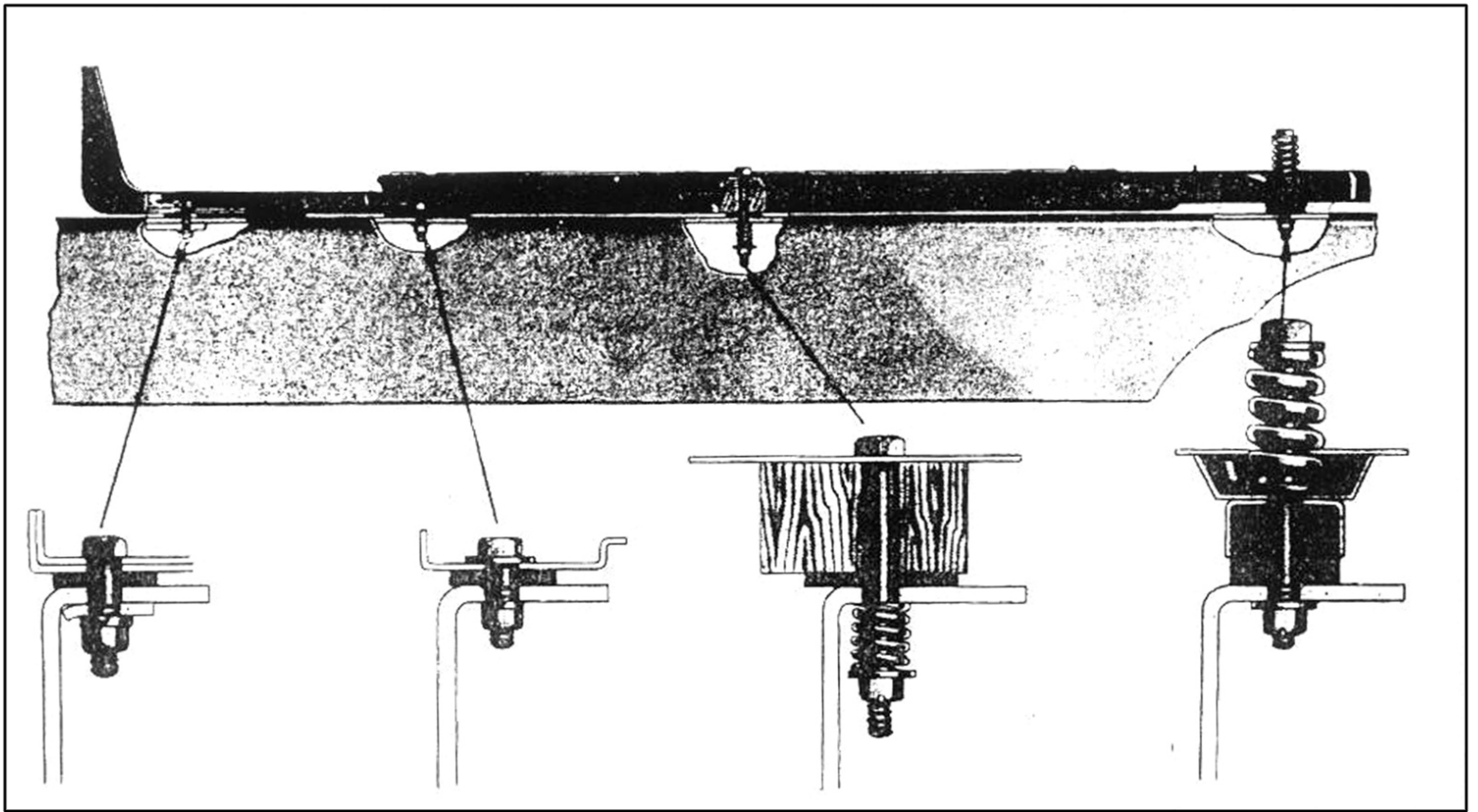
Fig. 84--Truck Cab Mounting
